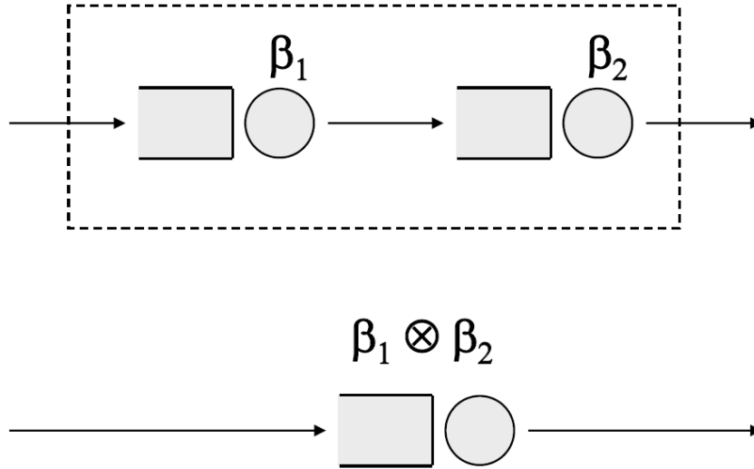
Figure 5: Illustrative example representing the concatenation of two nodes providing separate services into a single node providing an aggregate service, reprinted from [34]
