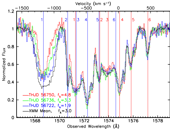
Figure 26. Illustration of variability in the narrow absorption components of C IV in NGC 5548 during the early part of the AGN STORM campaign, when the strength of C IV absorption in component 1 was highly correlated with the FUV continuum flux. Normalized relative fluxes are plotted as a function of velocity relative to the systemic redshift of z = 0.017175 for C IV \lambda 1548 . The colored curves are the spectra for the observation dates given in the key along with the observed flux at 1367 \text{ \AA} in units of 10^{-14} \text{ erg cm}^{-2} \text{ s}^{-1} \text{ \AA}^{-1} . The illustrated spectra show high (red), low (blue), and mean (green) flux levels in comparison to the mean spectrum from the XMM-Newton campaign (black). Vertical blue lines indicate the velocities of the blue components of the doublets for the six intrinsic absorbers. Vertical red lines show the locations of the corresponding red components. During AGN STORM, the absorption profile in component 1 varies as expected for gas showing an ionization response.
