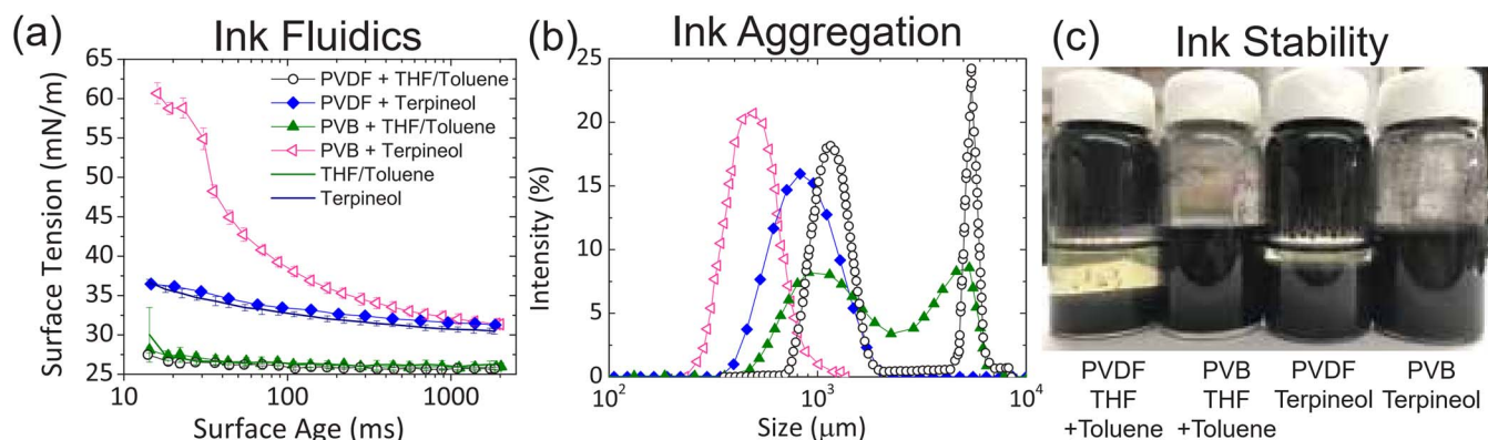
Figure 3. (a) Surface tension of PVDF in THF/Toluene, PVDF in Terpeneol, PVB in THF/Toluene, PVB in Terpeneol, THF/Toluene, and Terpeneol; (b) Particle size distribution of cathode materials in different systems; (c) Digital images of the four suspensions. They were standing for one day after preparation.
