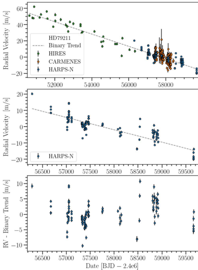
Figure 1. Radial velocities for HD 79211 measured from CARMENES (orange, top panel only), HARPS-N (blue, all panels), and HIRES (green, top panel only) spectra. For most data points, the uncertainty in the RV is smaller than the size of the point. We mark the binary trend, fit as a second-order polynomial, with a dashed line in the top and middle panels. The bottom panel shows the HARPS-N radial velocities with the binary trend subtracted. We use the HARPS-N RVs with the binary trend removed when calculating the correlation between RV and activity indicators (Figure 4), and when calculating periodograms (Figures 5, 6, 7, 8).
