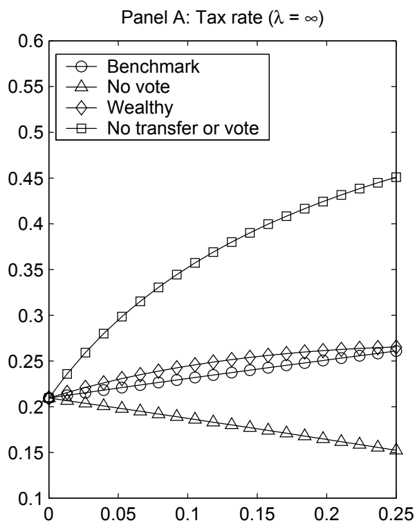
Figure 4: Results under various regimes
