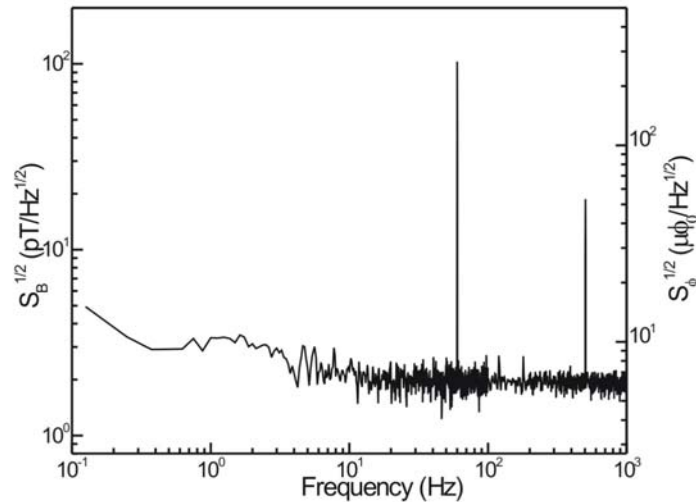
Figure 3.3: Field noise S_B^{1/2} and flux noise S_\Phi^{1/2} spectral density of one of our monolithic SQUID sensors
