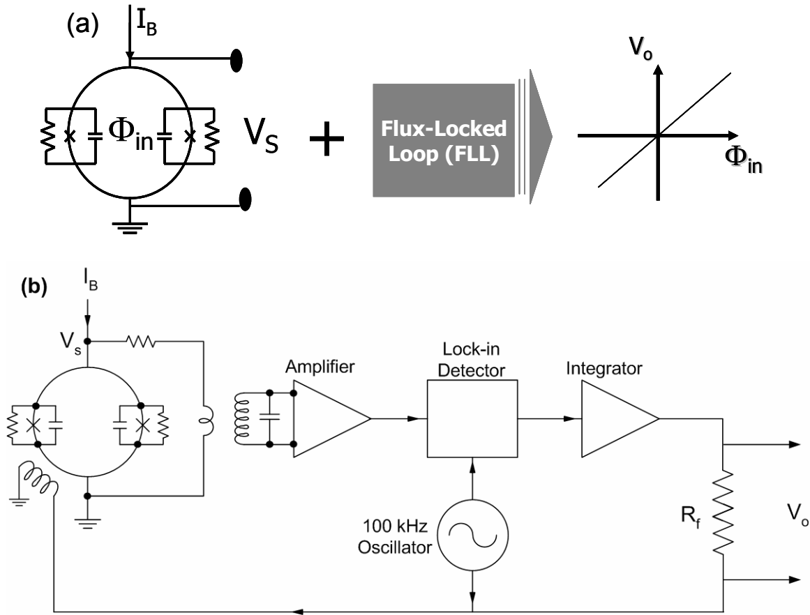
Figure 2.12: (a) The transfer function between the input magnetic flux \Phi_{in} and the voltage output of the SQUID V_s is nonlinear and periodic. In order to have a linear relationship, we operate the SQUID in a Flux-Locked Loop (FLL). (b) FLL modulation and feedback circuit (adapted from 102). The SQUID is coupled to the preamplifier via a cooled step-up transformer. The voltage response of the SQUID V_s is the input of the FLL, which uses a modulation flux scheme to maintain the SQUID at an extremum on the V-\Phi curve. The user measures a change in V_o , which is proportional to the amount of flux changed detected by the SQUID.
