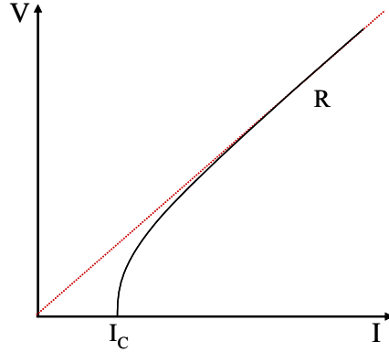
Figure 2.5: Single Josephson junction VI characteristic curve.
