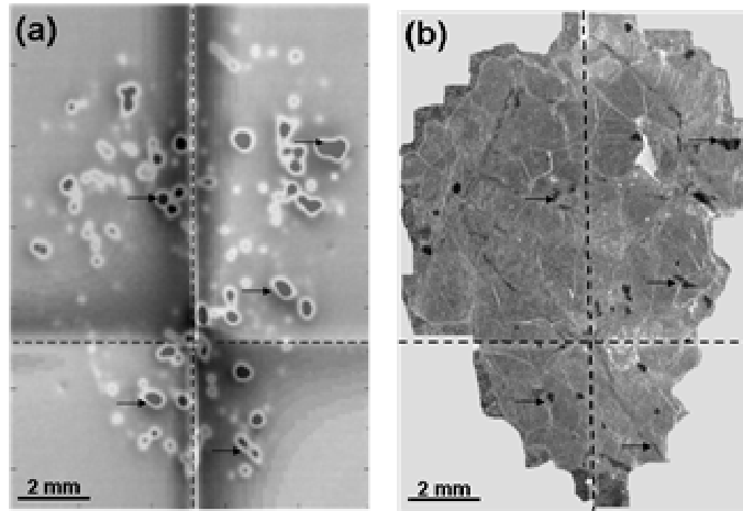
Figure 4.10: (a) Superposition of the magnetic field map from the sample and the magnetic field generated by wires across the sample used for registration purposes. (b) Optical picture of the sample. The dashed line shows the position of the wire. This registration technique allows us to correlate magnetic features with features in the optical image (arrows).
