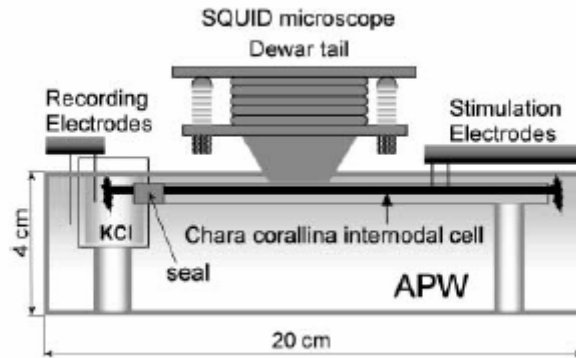
Figure 9.1: Schematic experimental setup ( side view ) used for electric and magnetic measurements on Chara corallina internodal cell. The Plexiglas holder supporting the cell is terminated on the left side in a sealed compartment to record the transmembrane potential.
