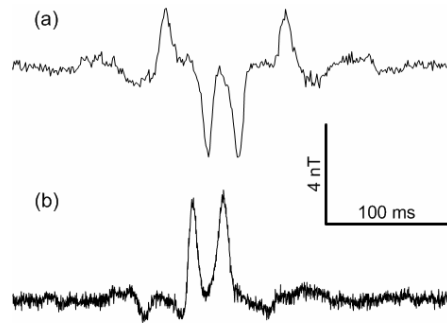
Figure 8.2: (a) and (b) Measured time traces of the magnetic field from two different magnetic particles moving through the serpentine channel.
