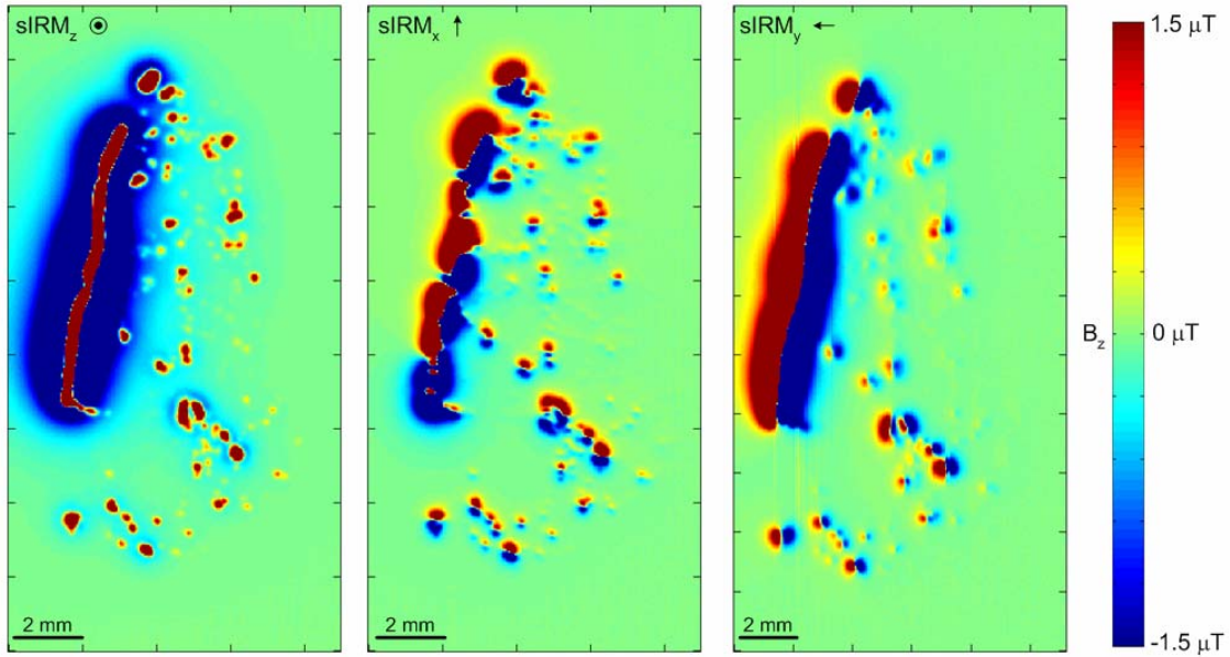
Figure 7.7: High resolution magnetic field maps of three-axis IRM saturation (sIRM) acquisition at a field of 545 mT
