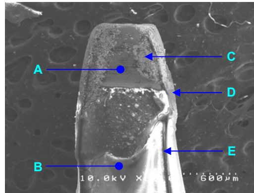
Figure 4.5: SEM image of a monolithic SQUID chip wired and mounted on the tip of a sapphire rod. (A) SQUID chip, (B) sapphire rod, (C) silver epoxy, (D) low-temperature epoxy resin (Stycast) and (E) gold wires connecting the SQUID to the electronics.
