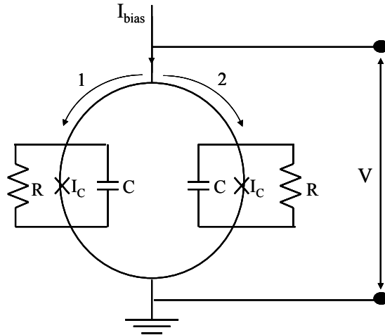
Figure 2.7: Schematic of a dc SQUID
