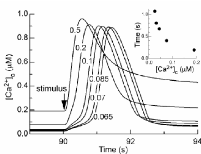
Figure 9.8: Simulated [Ca^{2+}]_c transients in response to a single electrical stimulation (100 ms/5 \mu A). Data were calculated with model parameters reported in Wacke et al. (2003) [20]. Different curves are obtained by changing the Hill coefficients \bar{p}_2 in the model term, which describes the buffering of [Ca^{2+}]_c . An increase in \bar{p}_2 over a range of 0.065 \mu M–0.5 \mu M results in reduced Ca^{2+} buffering and a consequent increase in the resting [Ca^{2+}]_c . In the simulation, pulses were started after 90 s in which the system was allowed to equilibrate. ( Inset ) Delay time between stimulus and maximal slope of [Ca^{2+}]_c increase as a function of resting [Ca^{2+}]_c before stimulation.
